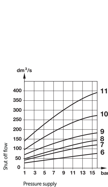
Flow ( \pm 10\% ) vs pressure supply (3/4 ... 1 1/2")
