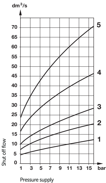
Flow ( \pm 10\% ) vs pressure supply (1/4 ... 1/2")
